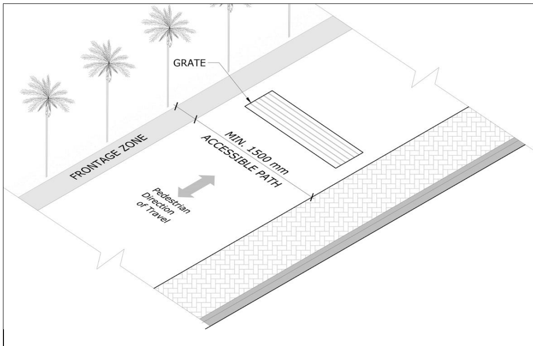
Figure 2. Grates in accessible routes
