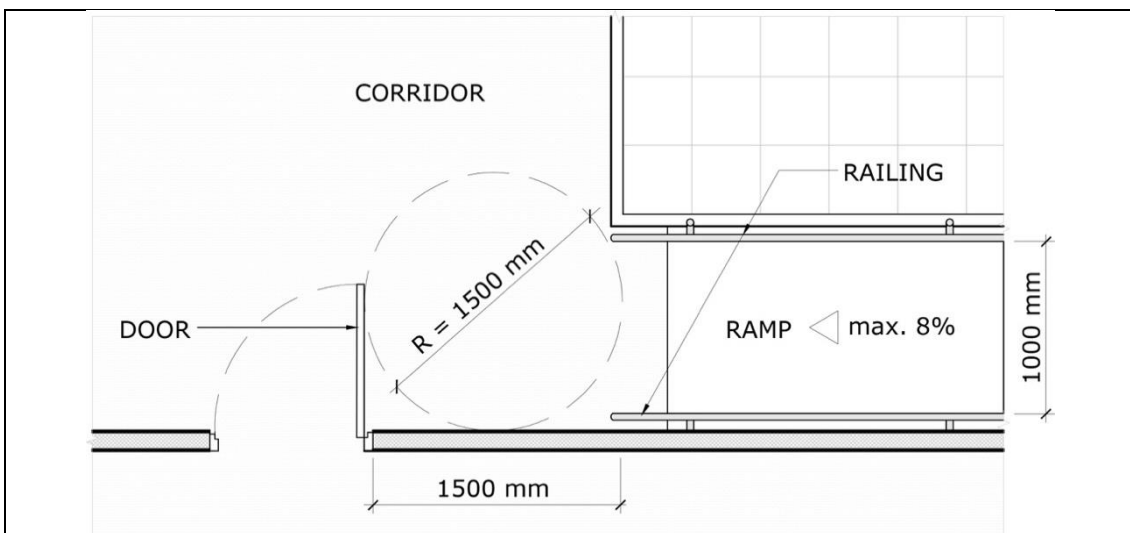
Figure 54. Clear space between ramp and doors
