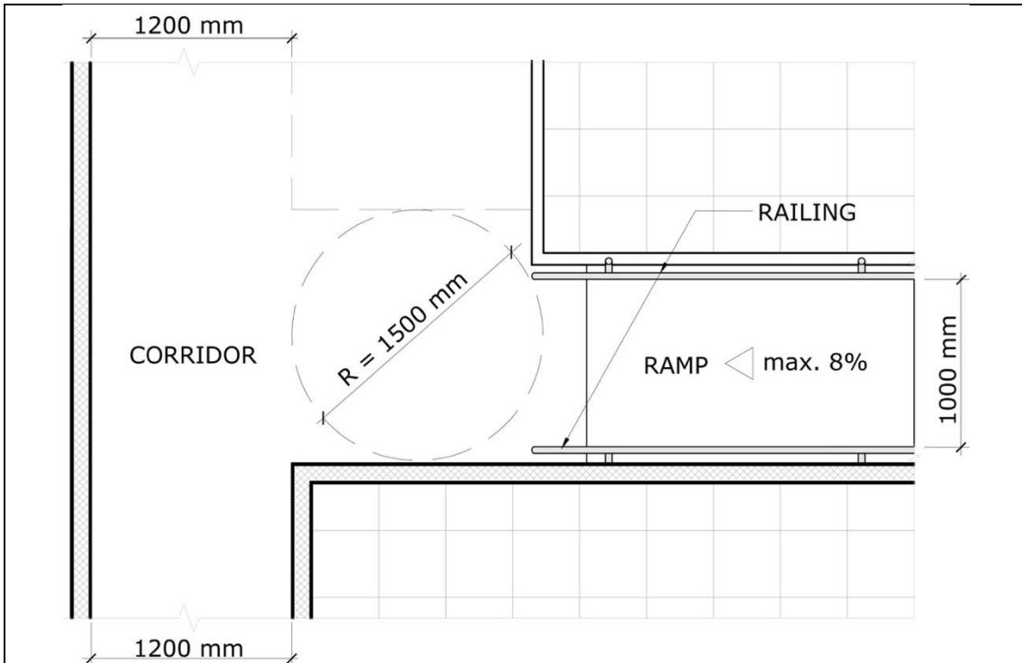
Figure 53. Intersection of ramp and corridor
