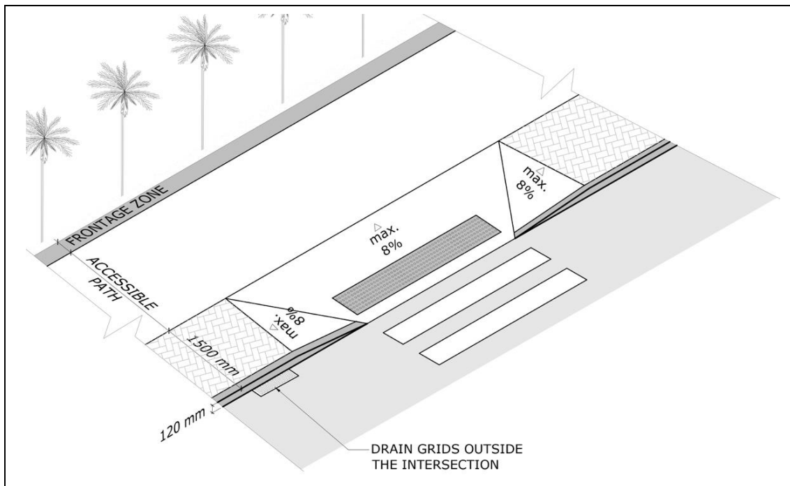
Figure 5. Kerb ramp with flared sides
