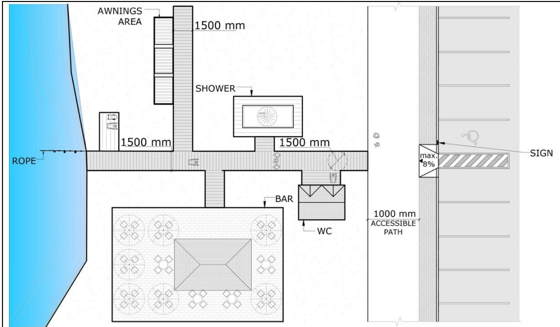
Figure 90. Accessible beach layout
