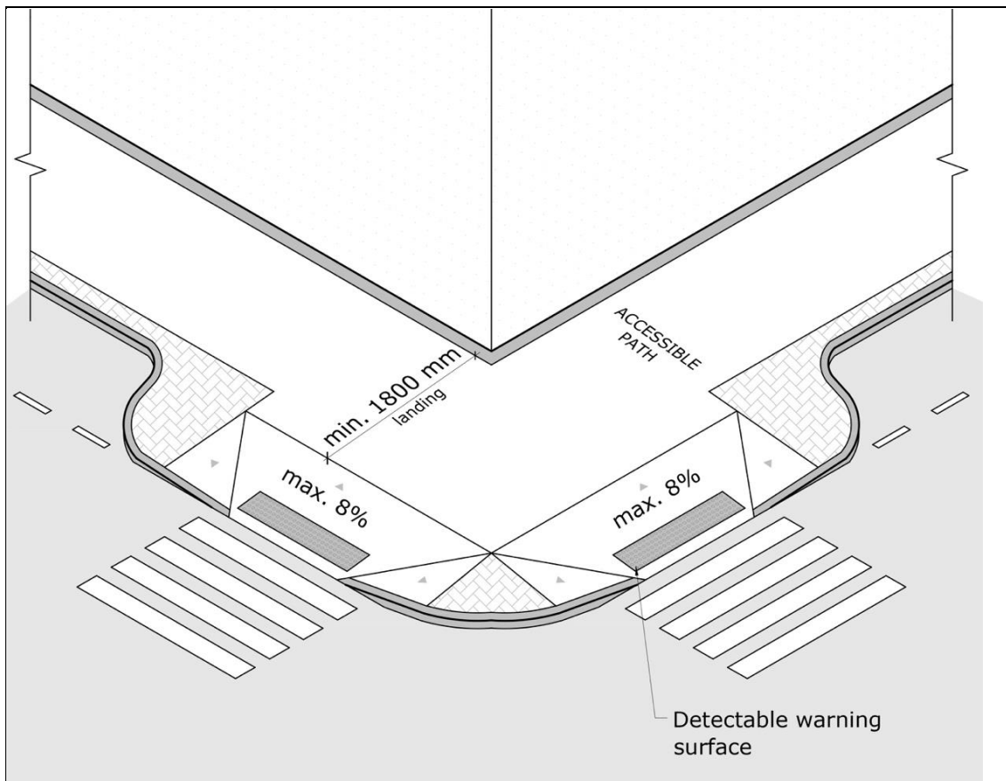
Figure 7. Kerb ramp in kerb extensions
