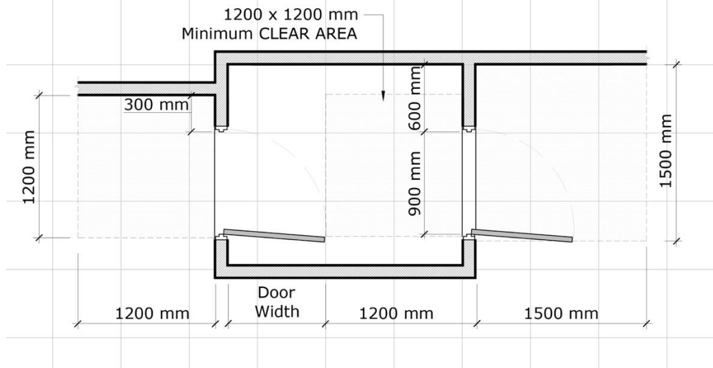
Figure 30. Door clear spaces
