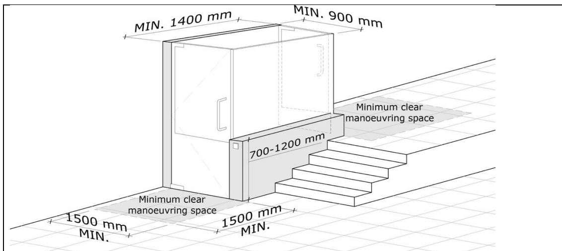
Figure 47. Specifications for non-enclosed platforms
