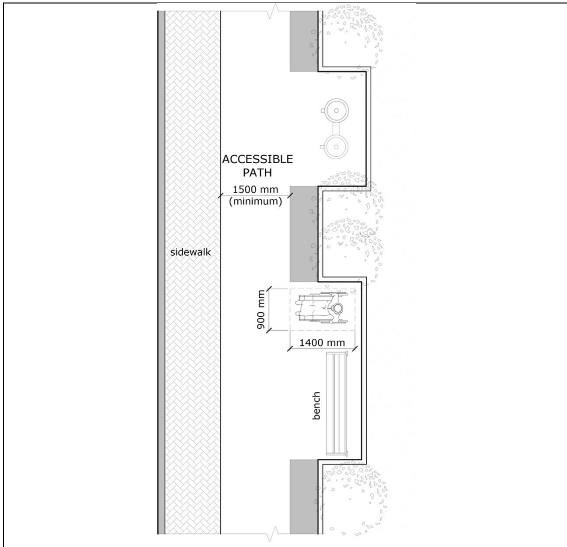
Figure 4. Accessible path with resting area example.
