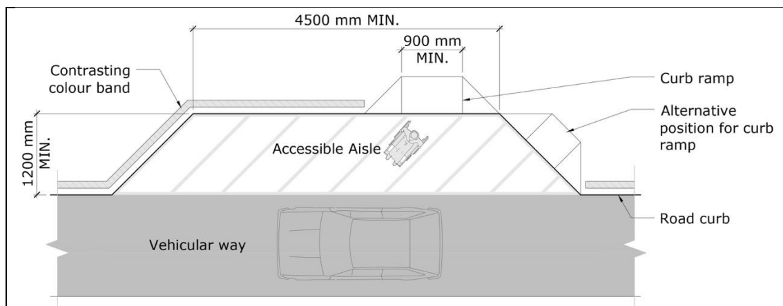
Figure 15. Pick-up area with kerb ramp
