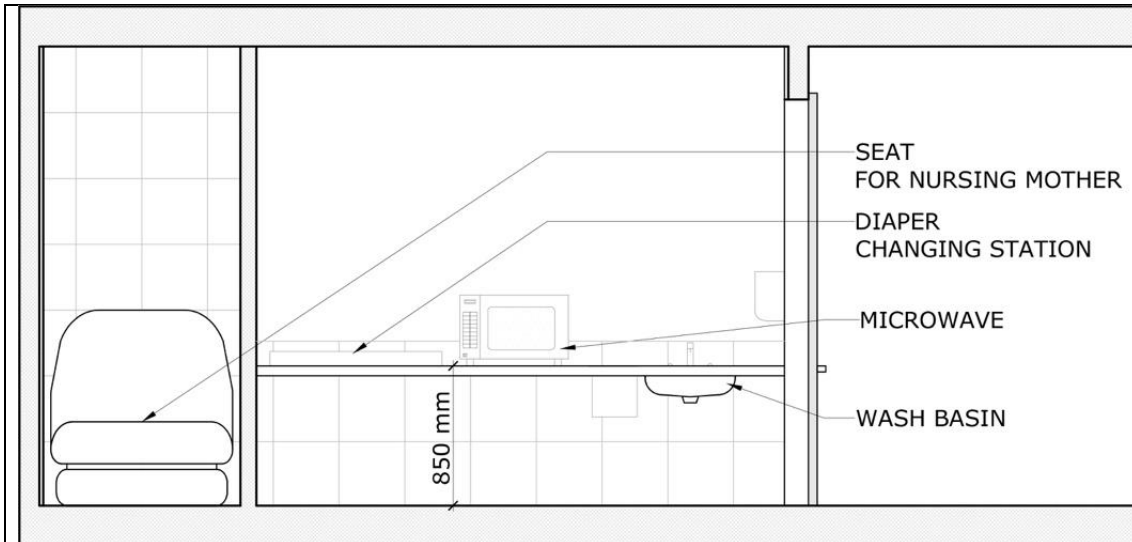
Figure 70. Feeding room option A, elevation.
