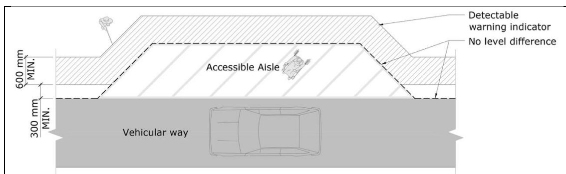
Figure 16. Pick-up area with no level difference
